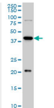
YY1 monoclonal antibody (M01), clone 2C4 Western Blot analysis of YY1 expression in HeLa S3 NE (Cat # AT4562a)
